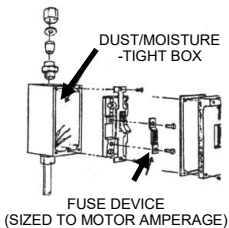
COMBINATION ON-OFF SWITCH AND MOTOR PROTECTIVE DEVICE
