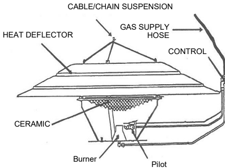
GAS BROODER STOVE
