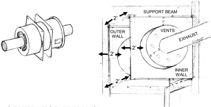
GENERATOR EXHAUST WALL PASS-THROUGH
