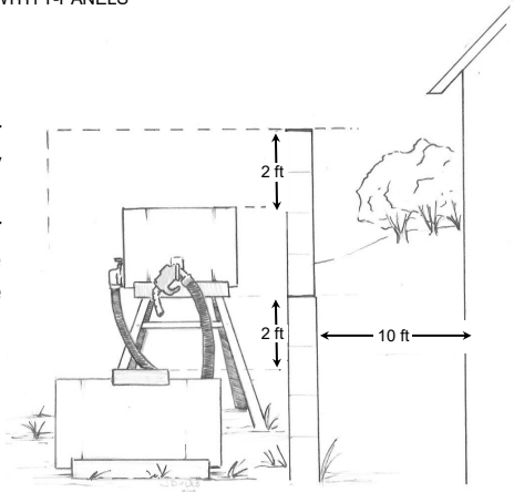
SIDE VIEW WITH BLOCKS
